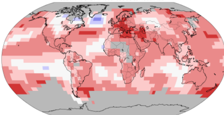
Land & Ocean Temperature Percentiles Jan–Dec 2018
